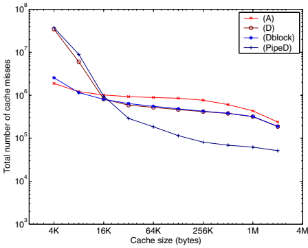
(c) MEDAKZO on one processor
