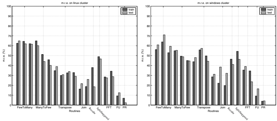
Fig. 7. Mean of relative errors (m.r.e.) on training set and test set
