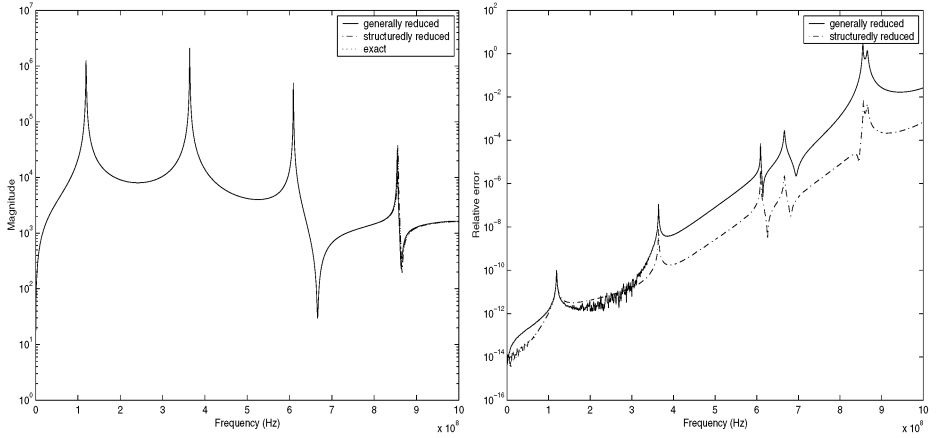
Fig. 2. Transfer functions (left) and relative errors (right)
