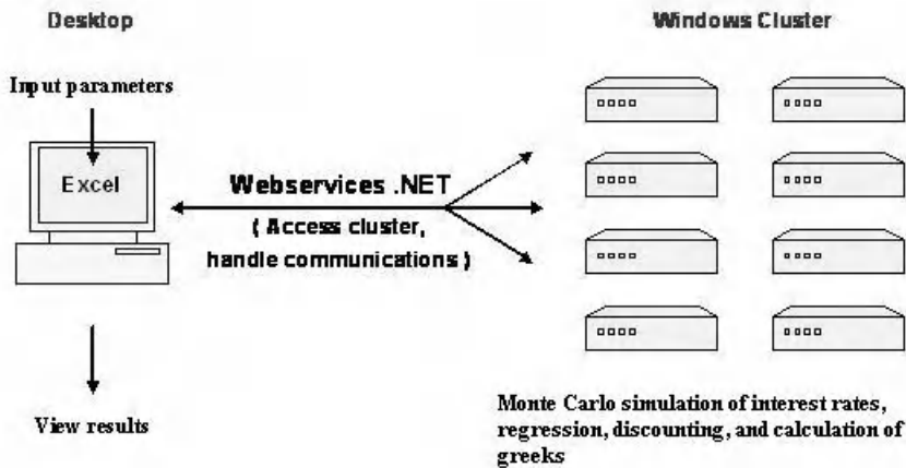
Fig. 1. Overview of computing architecture
