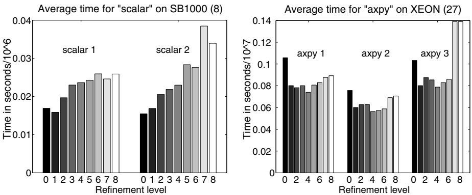
Fig. 3. Left: Average execution times for the operation scalar on different refinement levels (SB1000, 8 nodes per FE). Right: Average execution times for the operation axpy on different refinement levels (XEON, 27 nodes per FE)
