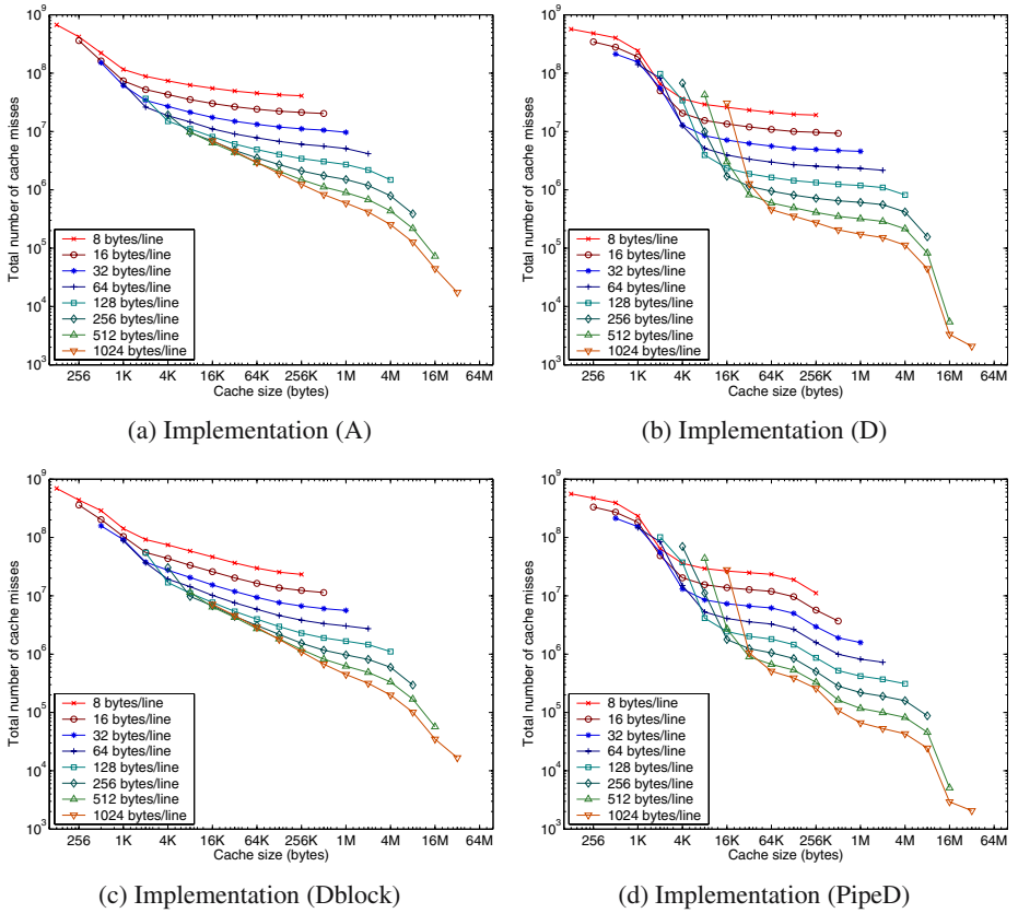
Fig. 3. Locality behavior for BRUSS2D for varying cache sizes and cache line sizes using one processor with a 16-way set-associative cache
