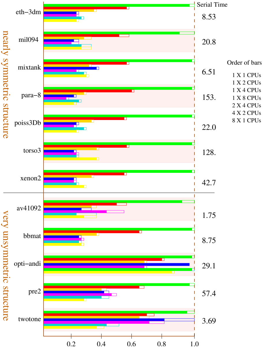
Fig. 5. WSMP factor and solve times from 1 to 8 CPUs (normalized w.r.t. single CPU time). The 8-CPU results are presented for four different configurations t \times p , where t is the number of threads and p is the number of MPI processes
