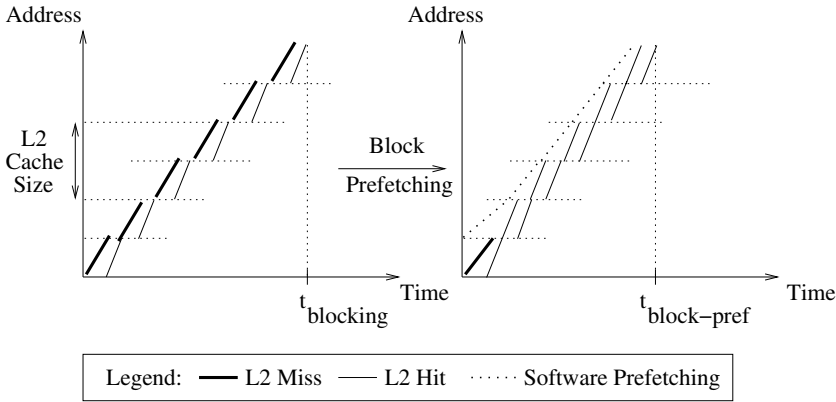
Fig. 2. The interleaved block prefetching transformation
