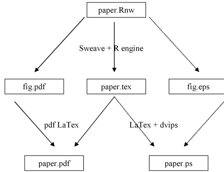
Fig. 2. The working principle of Sweave
