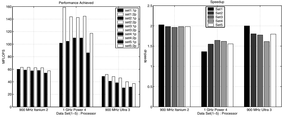
Fig. 2. Achieved Mflop rate and speedup The left graph shows the Mflop rate of the one-phase (1p) and two-phase (2p) schemes for the five matrix sets on an Itanium-2, a Power-4 and an Ultrasparc-3. The right graph shows the speedup of the one-phase scheme over the two-phase scheme for the same matrix sets on the 3 different platforms
