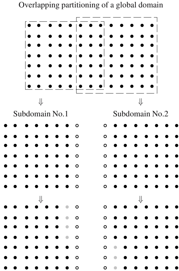
Fig.2. A simple example of reducing the number of computational points (black-colored) in two overlapping subdomains. The white-colored internal boundary points and the grey-colored overlapping points do not participate in the distributed global-level computations, these points receive computational results from the neighbor
