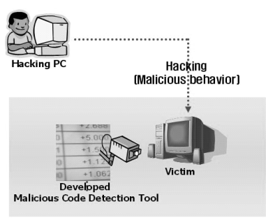
Fig. 6. Experiments architecture
