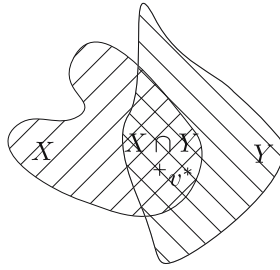
Fig. 4. Intersection stability
