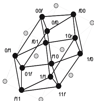
Fig. 2. The structure of DG(3) , where the dash line and dash node show the hypercube that is the DG(3) derived from
