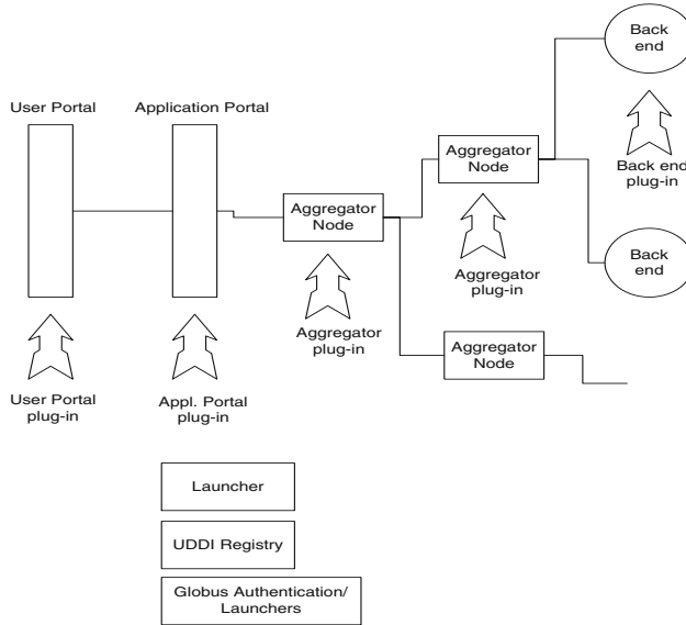
Fig. 1. Ygdrasil Infrastructure
