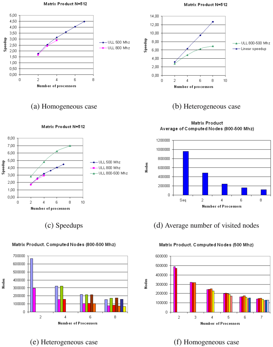
Fig. 5. Results for the Strassen's Matrix Multiplication
