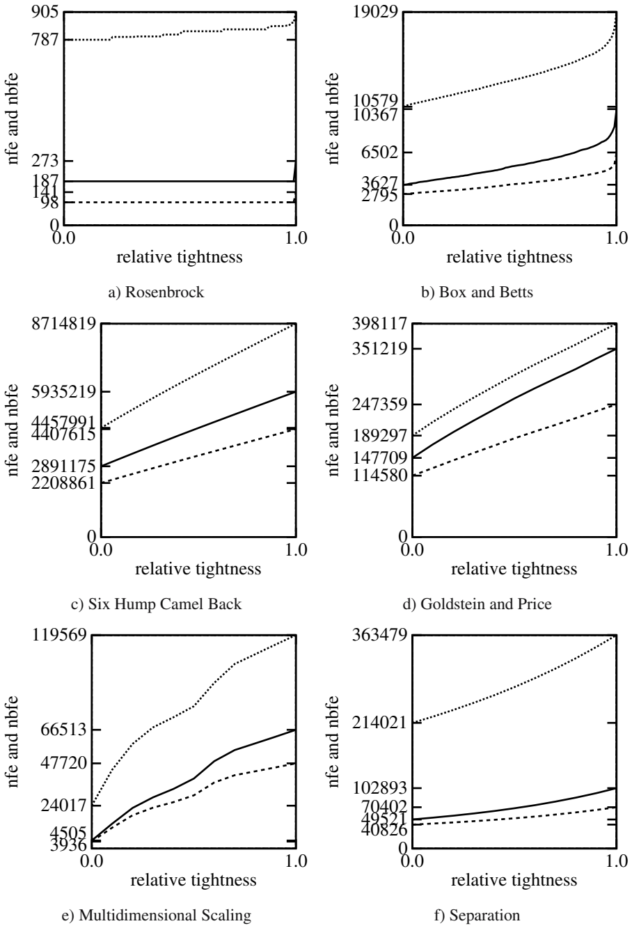
Fig. 2. Efficiency of tightening. Solid line represents numbers of bounding function evaluations and dashed line represents numbers of real function evaluations for the case ‘interval and real’, dotted line represents numbers of bounding function evaluations for the case ‘interval only’
