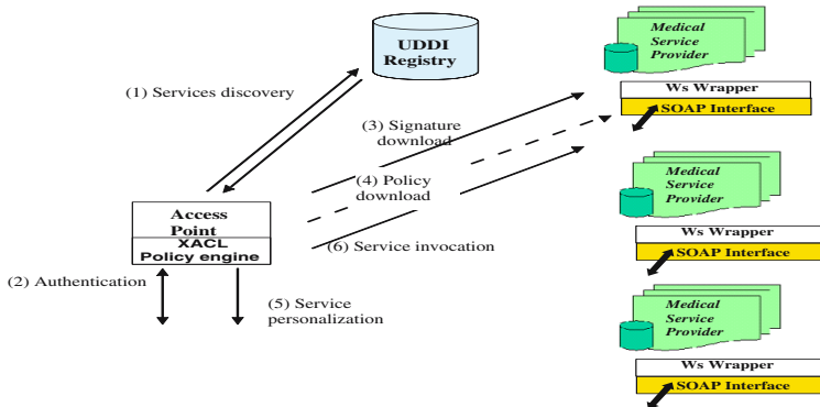
Fig. 5. Service exploitation in the implemented prototype
