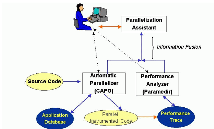
Fig. 1. Architecture of the expert system programming environment. The Parallelization Assistant Expert System fuses program structure knowledge and performance trace information to aid the user in narrowing down performance problems. The user can still interact directly with the parallelization and performance analysis tools for fine tuning of the application's performance
