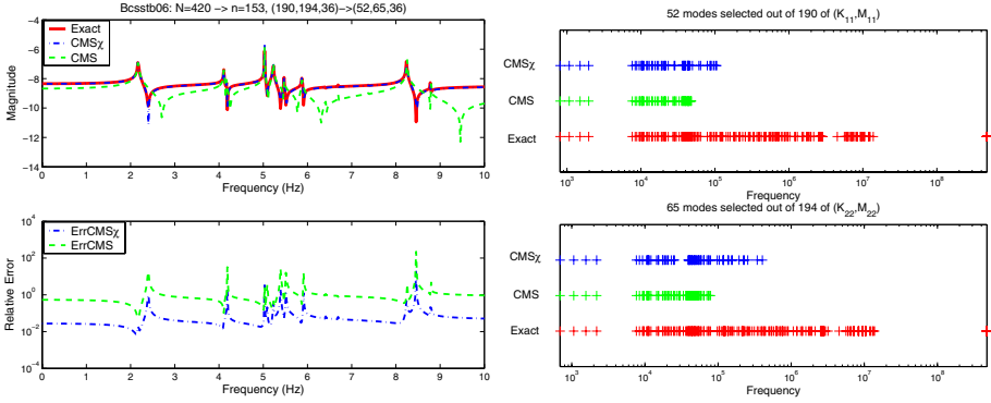
Fig. 2. Left: magnitudes (in log of base 10) of the transfer functions (top) and relative errors (bottom). Right: retained modes of subsystems by CMS and \text{CMS}_\chi
