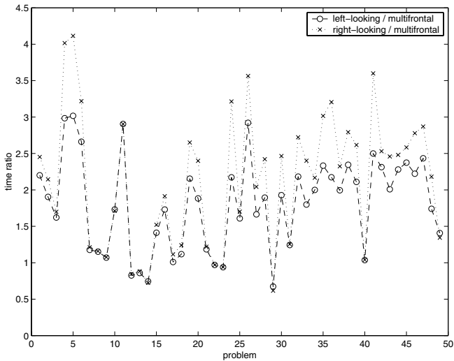
Fig. 3. The ratios between the execution times of the left-looking and multifrontal algorithms, and between the execution times of the right-looking and multifrontal algorithms, \tilde{L}\tilde{L}^T factorization (IBM Power 3 platform: 375 MHz, 16 GB)
