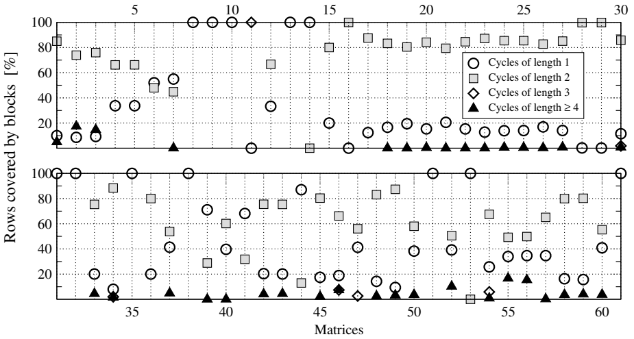
Fig. 1. Distribution of the cycle lengths for the tested matrices. Upper chart: matrices 1-30, lower chart: matrices 31-61
