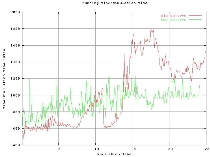
Fig. 6. Simulation runtime
