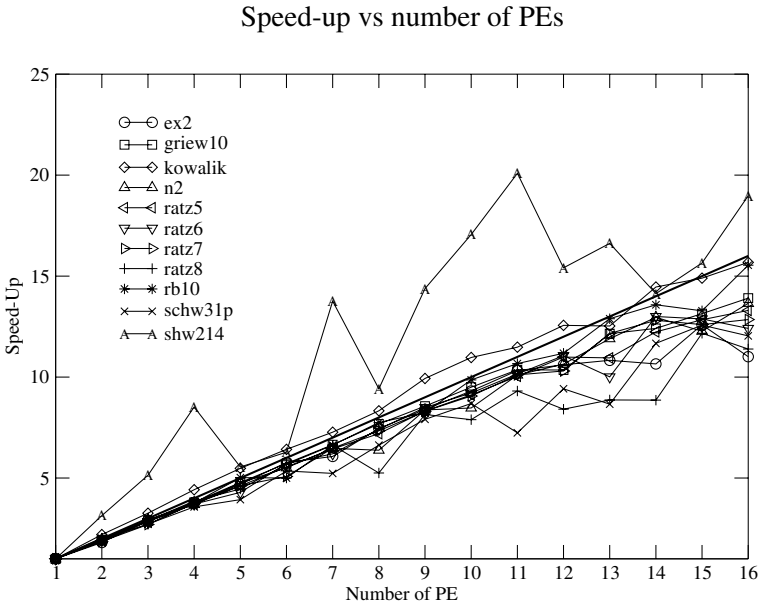
Fig. 1. Speed-up
