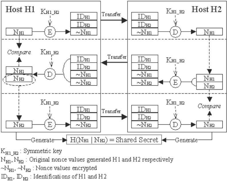
Fig.2. Mutual Authentication Process between Hosts
