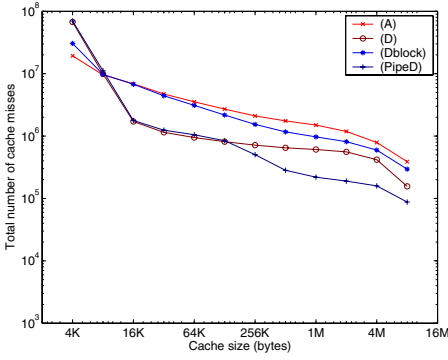
(a) BRUSS2D on one processor
