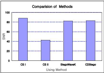
Fig. 11. Comparison of SNR(dB) between Cover-data and Stego-data
