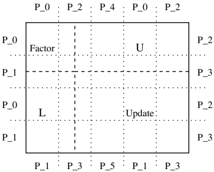
(b) A partial factor and update task mapped onto a 6-process 2-dimensional grid.
