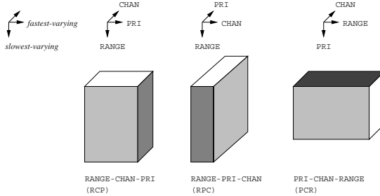
Fig. 3. Different orientations
