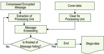
Fig. 2. Message Embedding FlowChart
