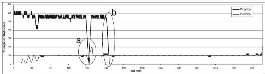
Fig. 3. Experiment M=10000 B=400 LdnAvgTput = 50KB/s : communication throughput along the time
