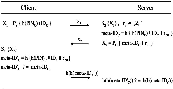
Fig. 1. Registration phase
