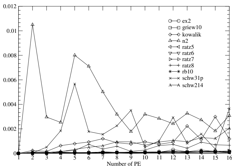
Fig. 2. Workload imbalance
