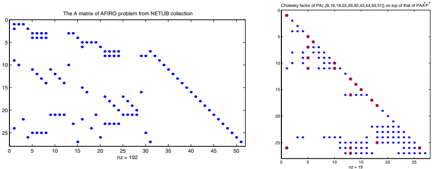
Fig. 1. Sparse structures
